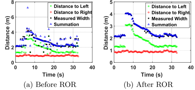
Figure 12: After ROR, outliers are removed, and all measured width and summation pairs match well.
