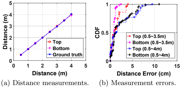
Figure 7: Distance candidate accuracy and error for both top and bottom microphones.
