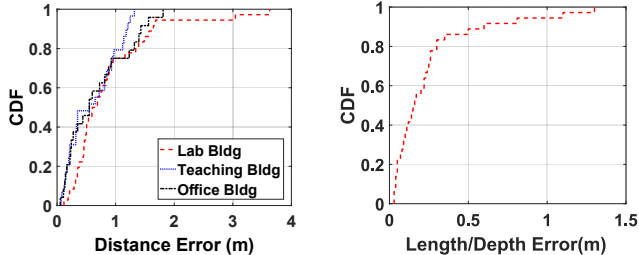
Figure 15: CDF of door location errors for three buildings.
