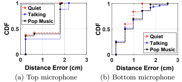
Figure 8: CDF for measurement errors of both microphones in different scenarios: quiet room, human talking, and pop music at a fixed distance of 3.5 meters.
