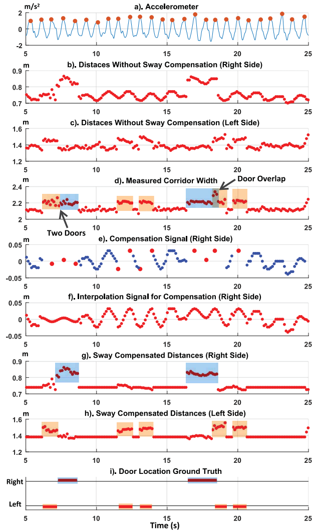
Figure 5: Phone sway while walking and compensation.
